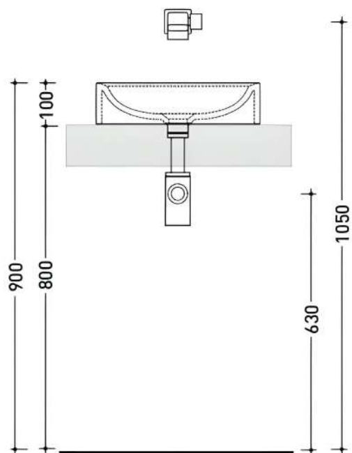
vista frontale / frontal view
