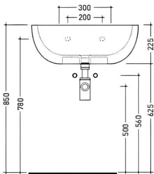
vista frontale / frontal view
